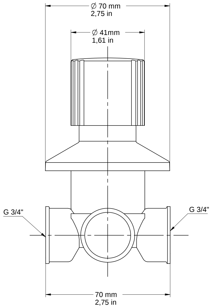
MISTURADOR AF/AQ PAREDE PRESSMATIC WALL-MOUNT MIXER VALVE W/ TRIM AND HANDLE MEZCLADOR PARED LAVATORIO
